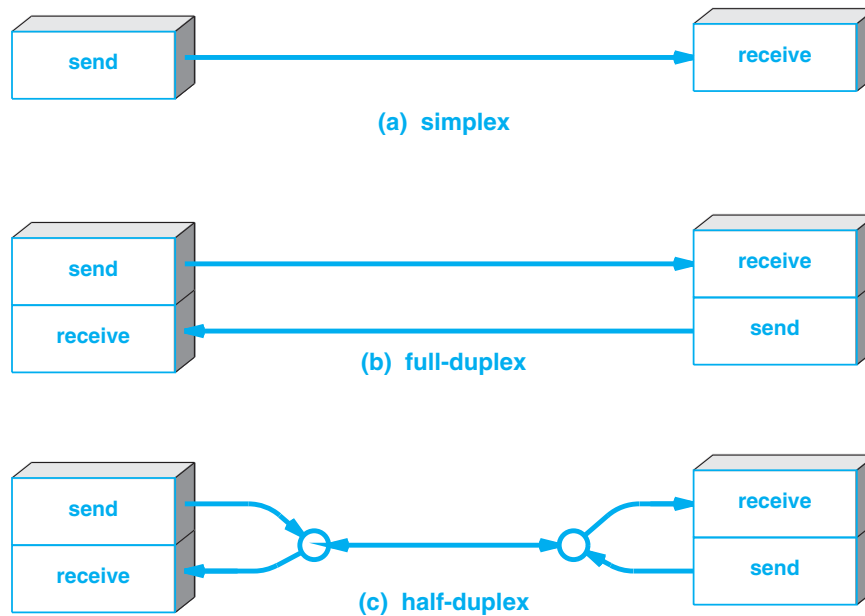
Figure 9.8 Illustration of the three modes of operation.
