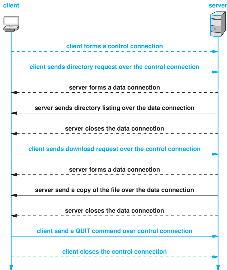
Figure 4.10 Illustration of FTP connections during a typical session.
