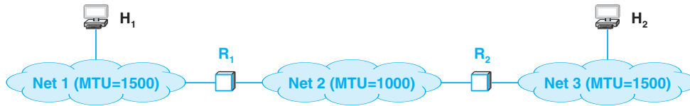
Figure 22.12 Illustration of three networks connected by two routers.
